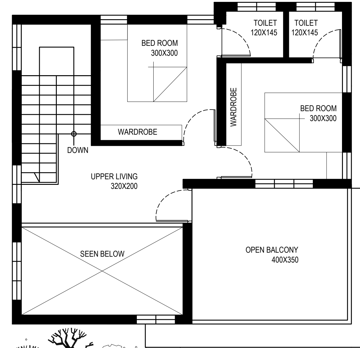
FIRST FLOOR PLAN FF AREA - 479 SQFT
