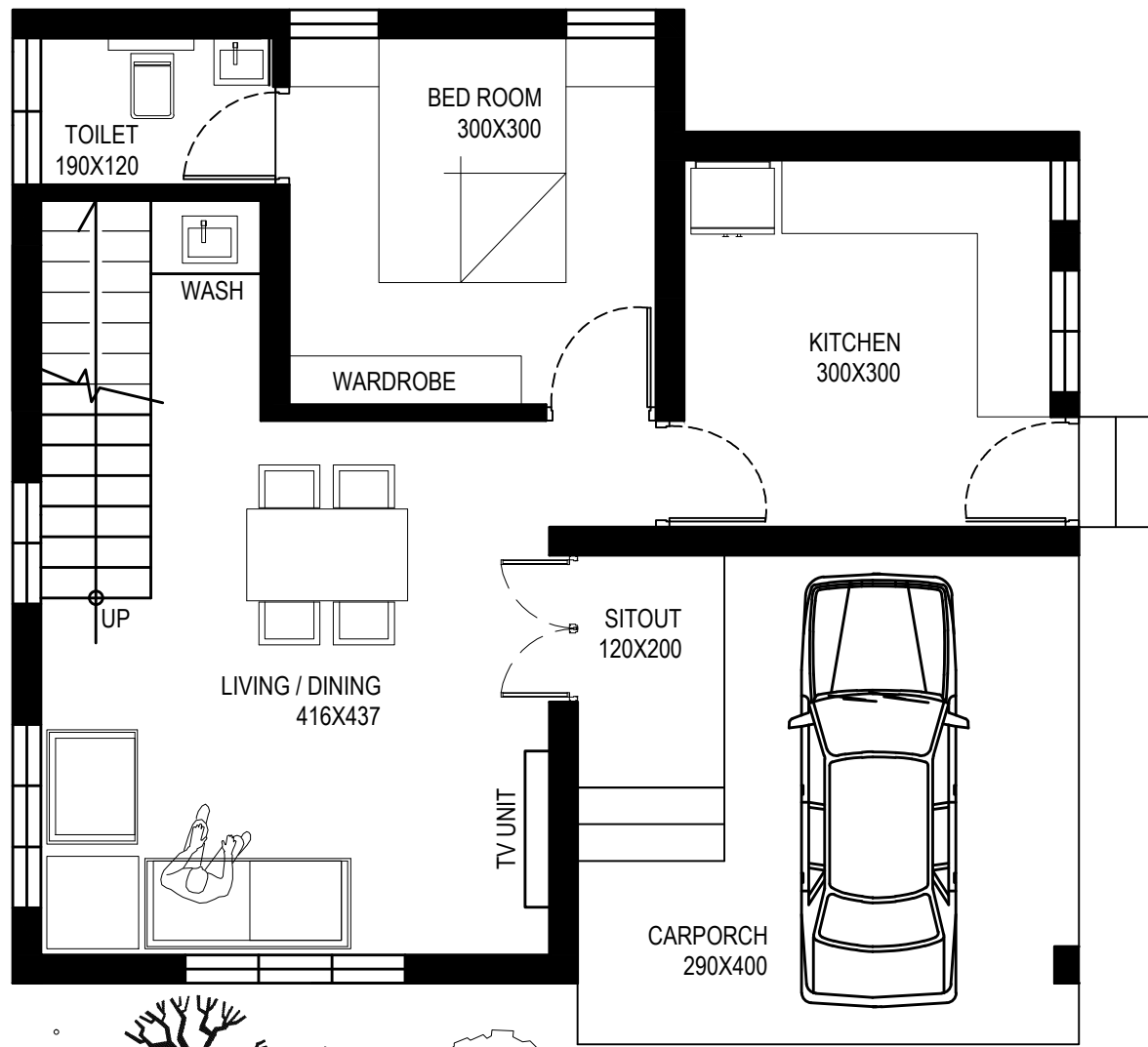
GROUND FLOOR PLAN GF AREA - 557 SQFT CAR PORCH AREA - 178 SQFT
